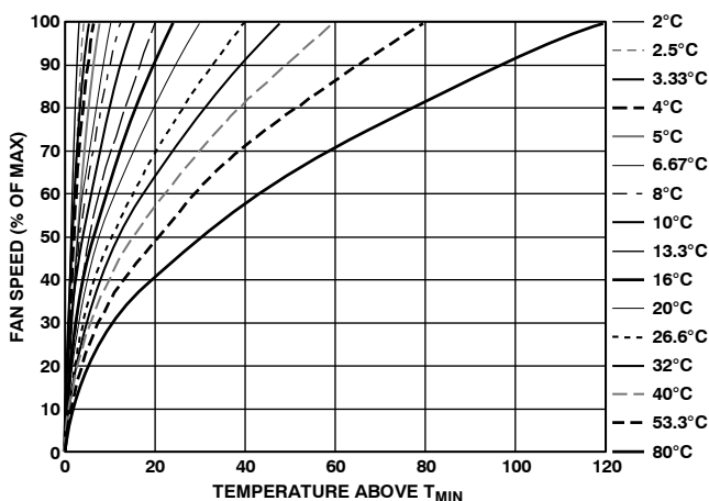
Figure 61. T_{RANGE} VS. Actual Fan Speed Profile
