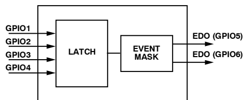
Figure 85. EDO Circuit
