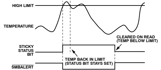
Figure 39. ALERT and Status Bit Behavior
