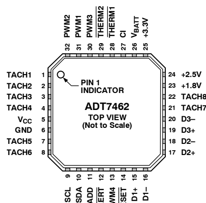
Figure 4. Configuration Option 1
