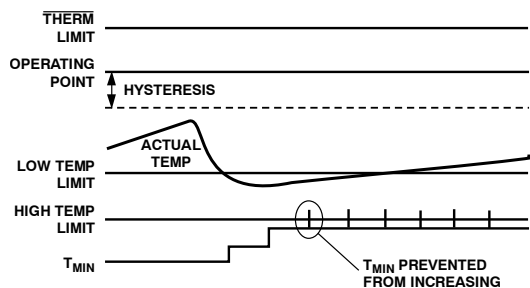
Figure 74. T_{MIN} Adjustments Limited by High Temperature Limit
