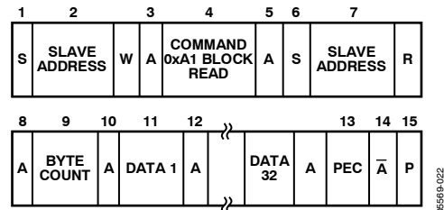
Figure 32. Block Read from RAM
